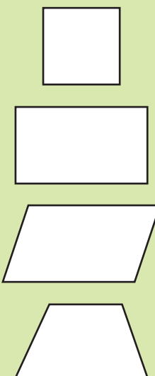
Trapez
