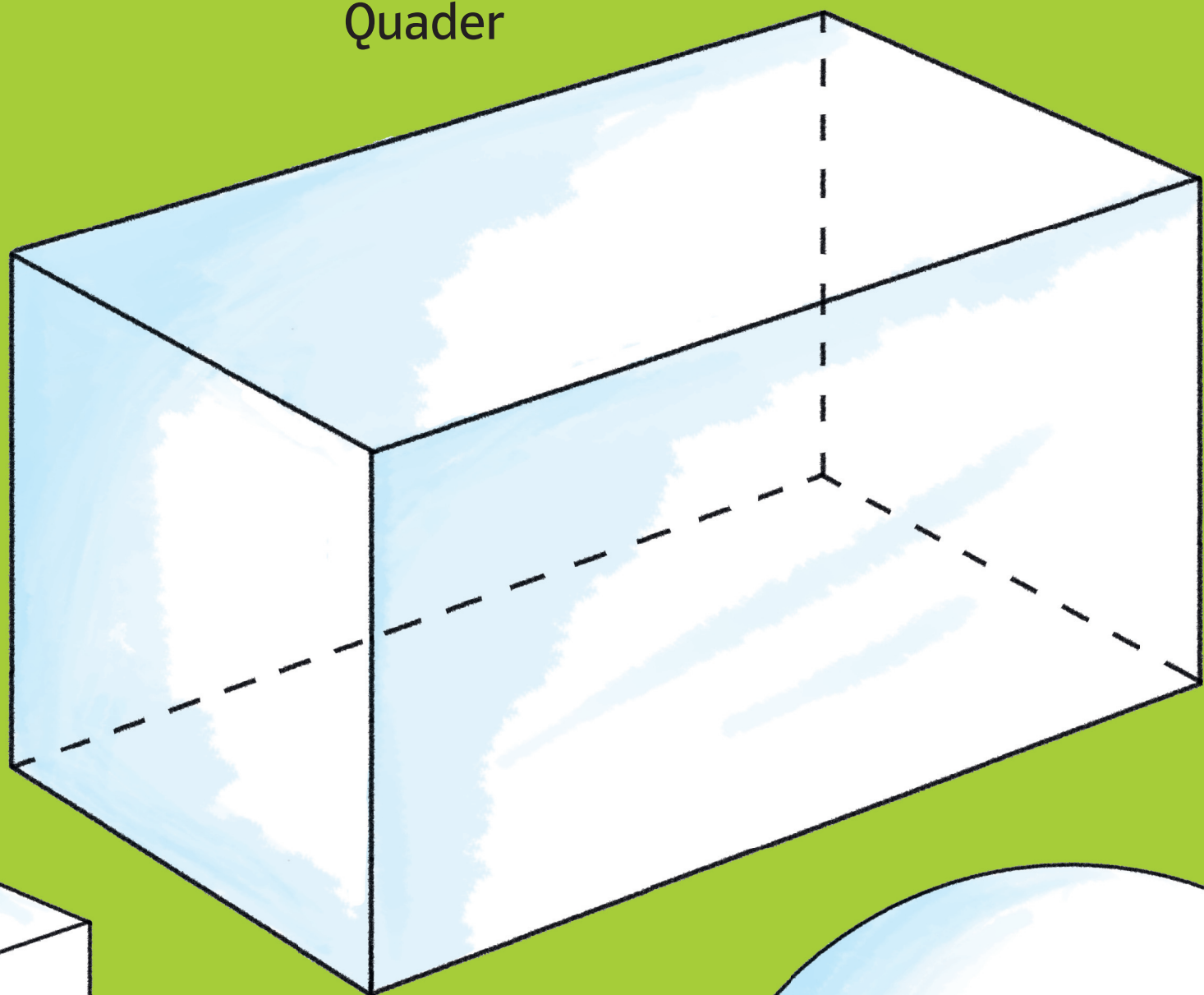
Quader
